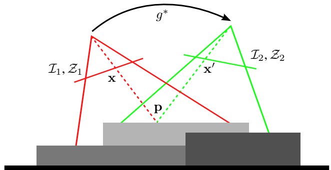
Fig. 2: The general idea of our dense RGB-D alignment approach: We estimate the camera motion g^* between two RGB-D images by minimizing photometric and the geometric error.
